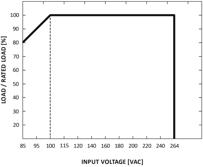
ⓈSTATIC CHARACTERISTIC
