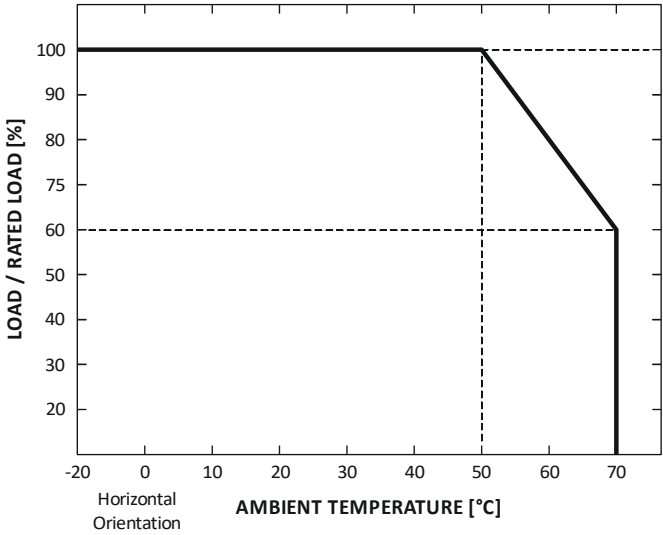
ⓈDERATING CURVE
